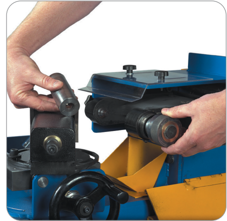
Patented quick-change roller system
