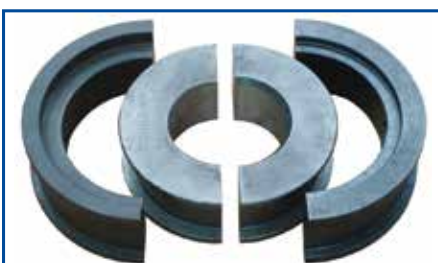
Clamp die interface kits necessary for flanging tube sizes \text{Ø} 20 \text{ mm} - \text{Ø} 219.1 \text{ mm} supplied with machine.
